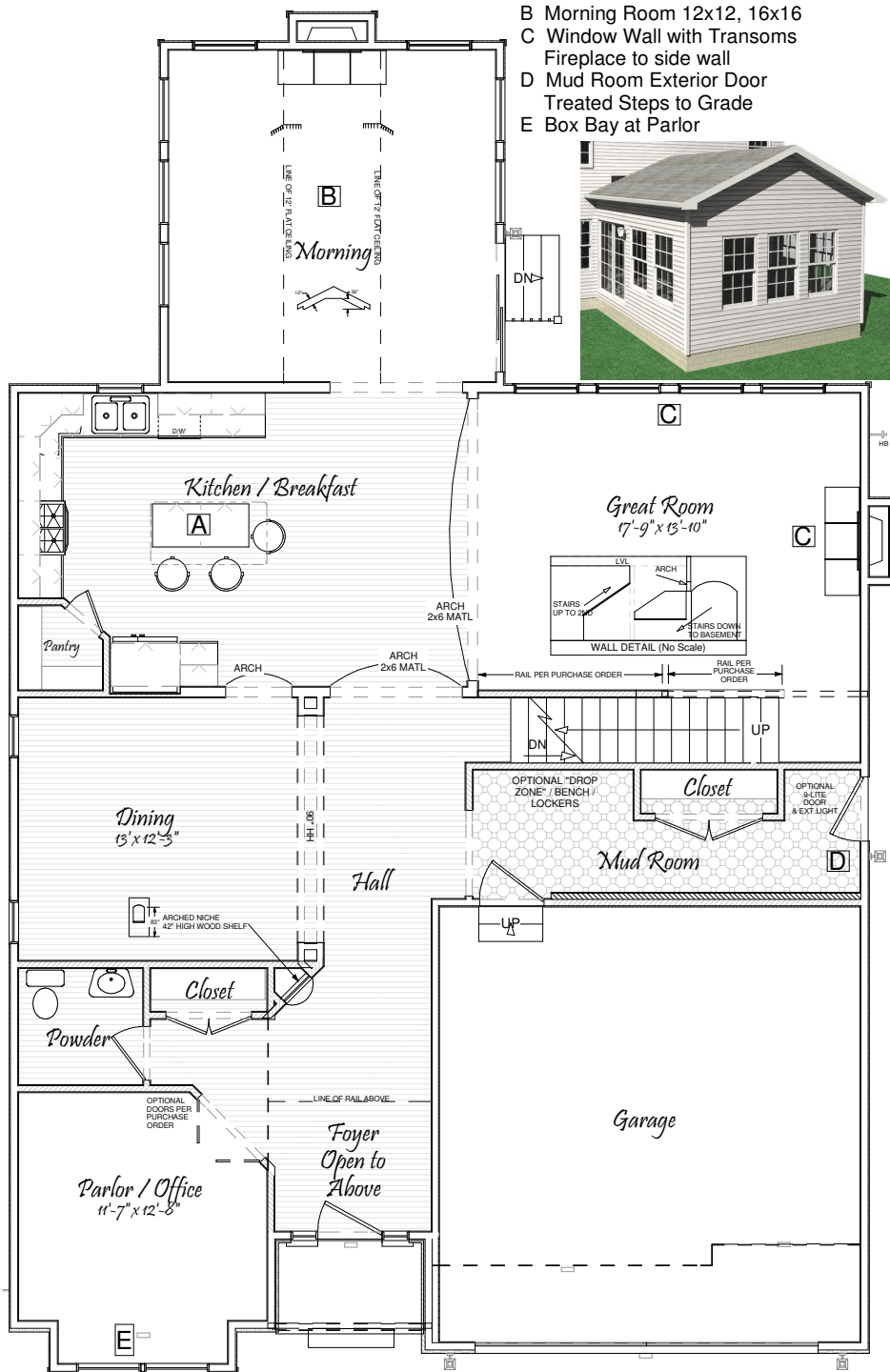
1st Floor Options
