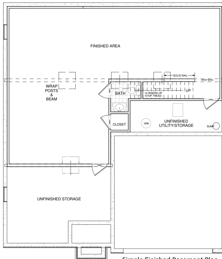
Simple Finished Basement Plan
