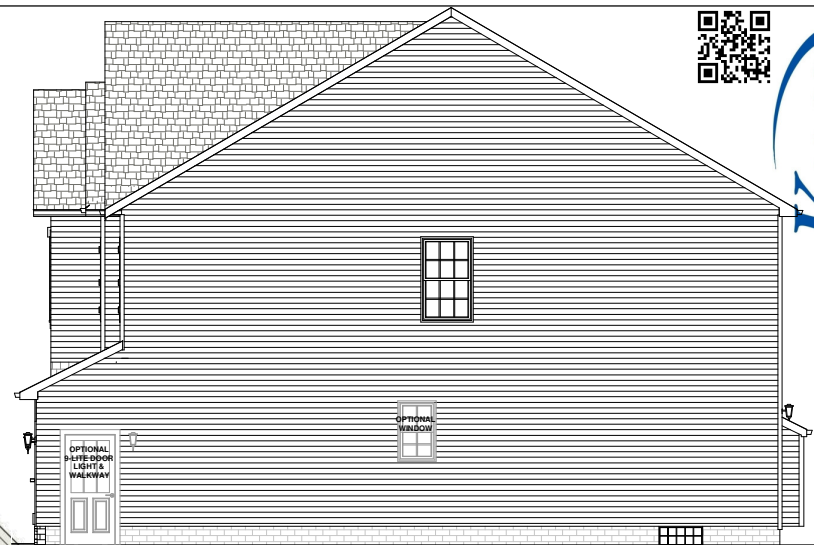
RIGHT GABLE ELEVATION
